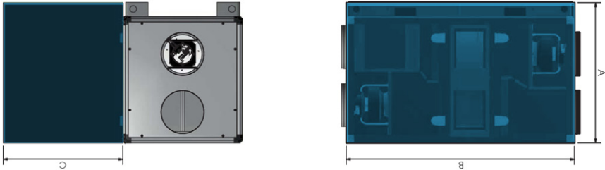
*Minimum spaces required for the ordinary maintenance (in mm).
